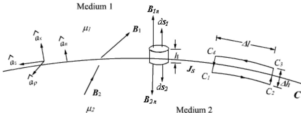
Figure 4.9: Interface between two magnetic media
